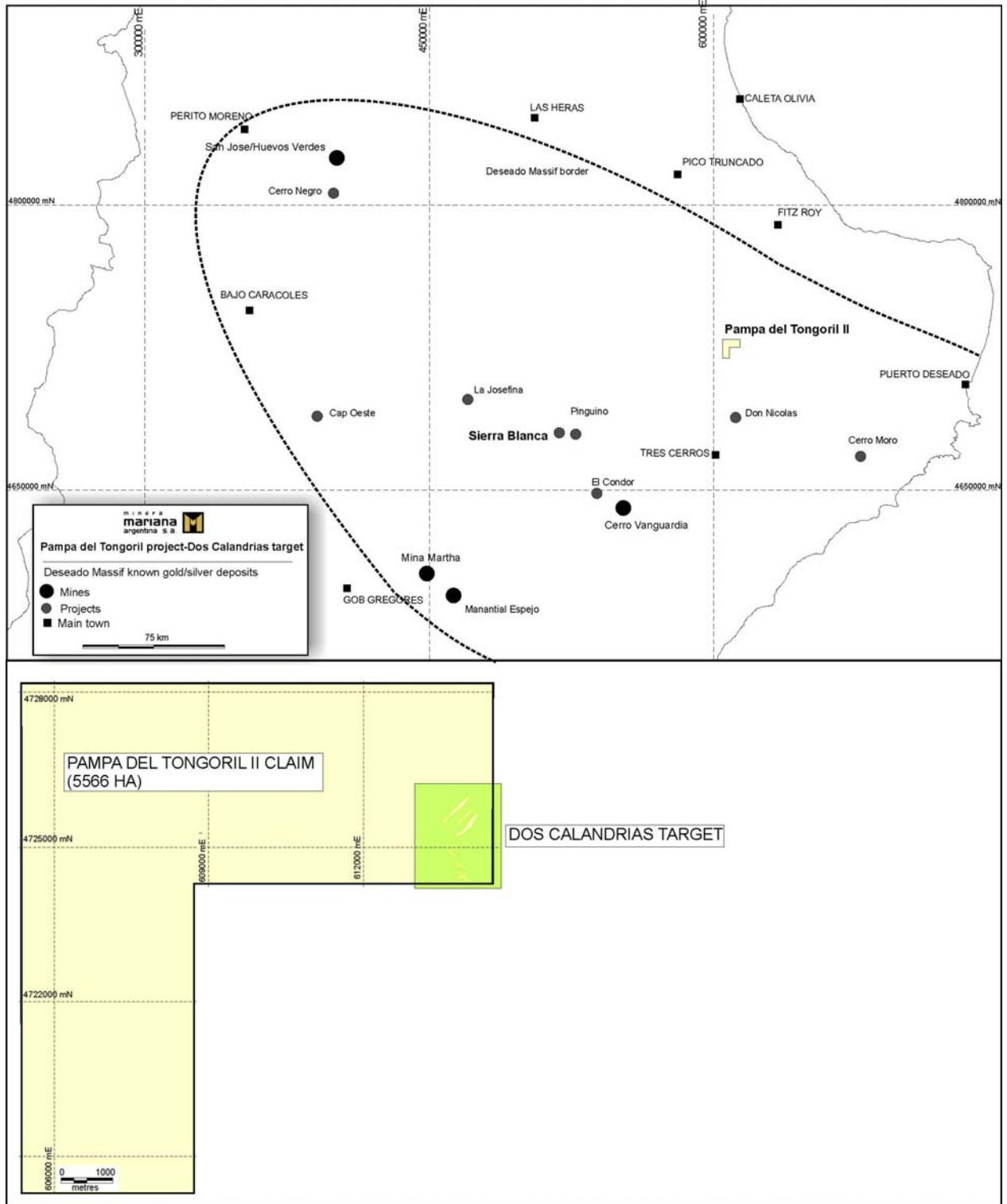
Figure 1: Deseado Massif and location of Dos Calandrias Project.
